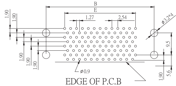
P.C.BOARD LAYOUT PATTERN
