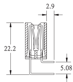
(CLOSE TYPE)
